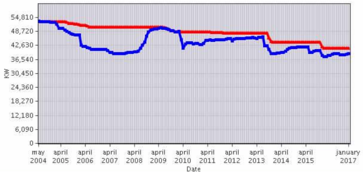
Cyprus: Power of the fleet compared to its power ceiling. Evolution between 1-5-2004 and 1-1-2017. (power ceiling: red line)
