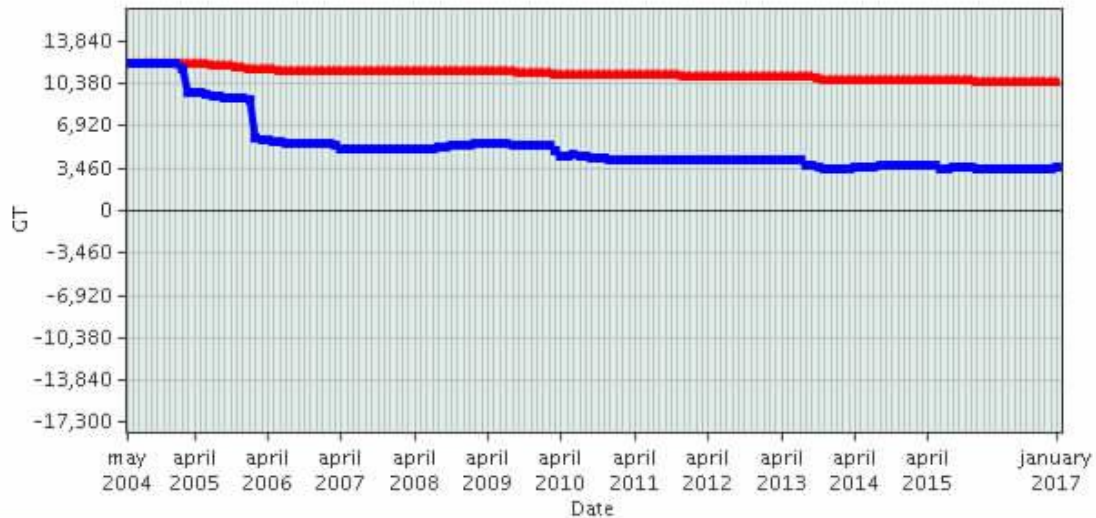
Cyprus: Tonnage of the fleet compared to its tonnage ceiling Evolution between 1-5-2004 and 1-1-2017 (tonnage ceiling: red line)
